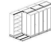
Front 3 Layers, Mid 3 Layers & Back 4 Layers Sliding Cabinet SC-CNN34306142016 3664W x 1420D x 160H/mm SC-CNN34406142016 4064W x 1420D x 160H/mm
